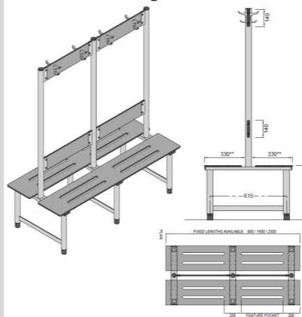
Island benching
