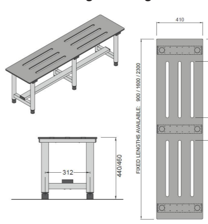
Freestanding benching
