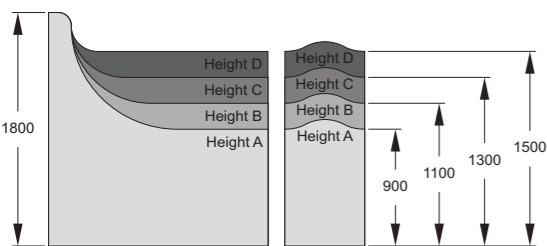
Door and partition height options
