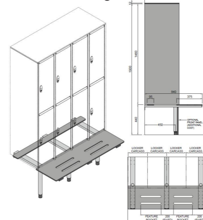
Locker benching
